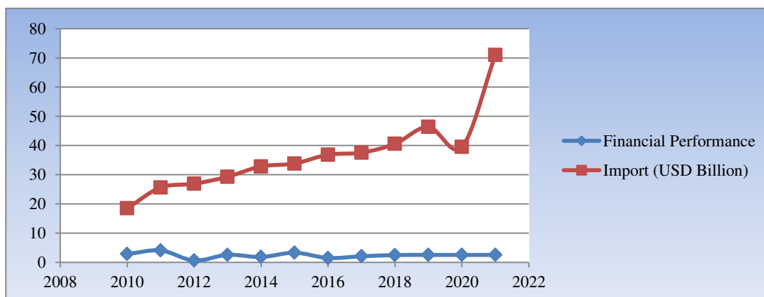
Fig. 2: Scatter plot for financial performance and import.
