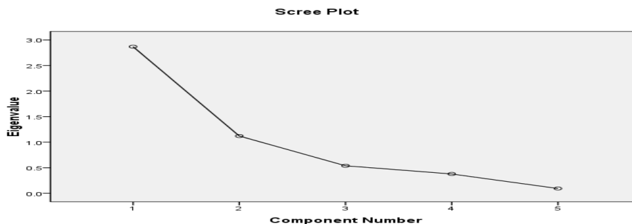
Fig. 6: Graph-based calculation of the ideal number of components.
