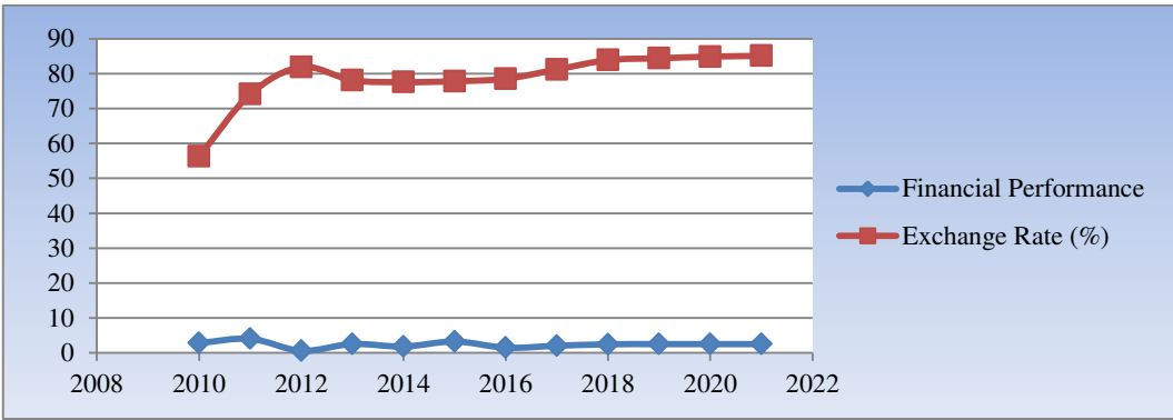
Fig. 5: Scatter plot for financial performance and exchange rate.
